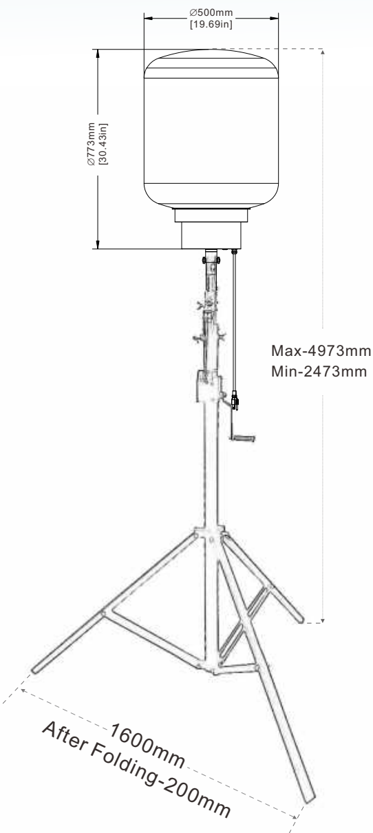
4.3m Tripod
