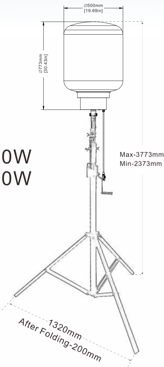
3m Tripod
